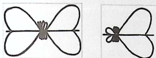
Long-wire Beverageantenn Figur 2. Horisontella strålningsdiagram
